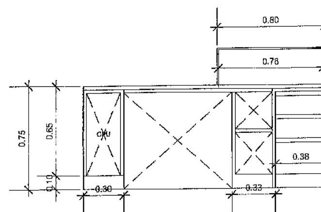
F-04 BACK VIEW 1:25
