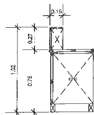
F-04 SIDE VIEW 1:25
