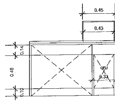
F-03 BACK VIEW 1 : 25
