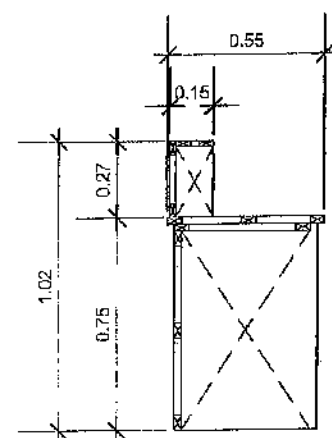
F-03 SIDE VIEW 1 : 25
