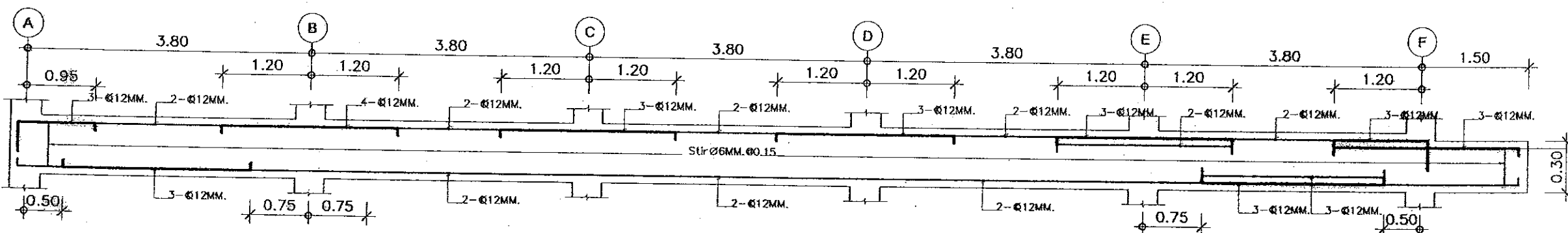
B7 (0.20x0.30, 0.20x0.40)
