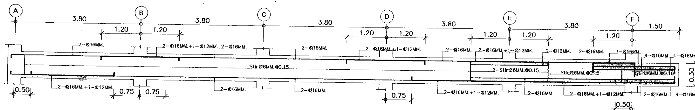
B6 (0.20x0.30, 0.20x0.40)
