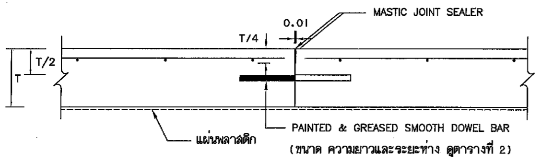
CONSTRUCTION JOINT
