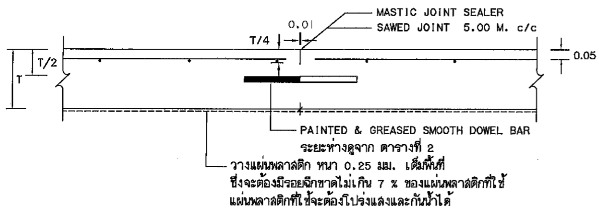
CONTRACTION JOINT
