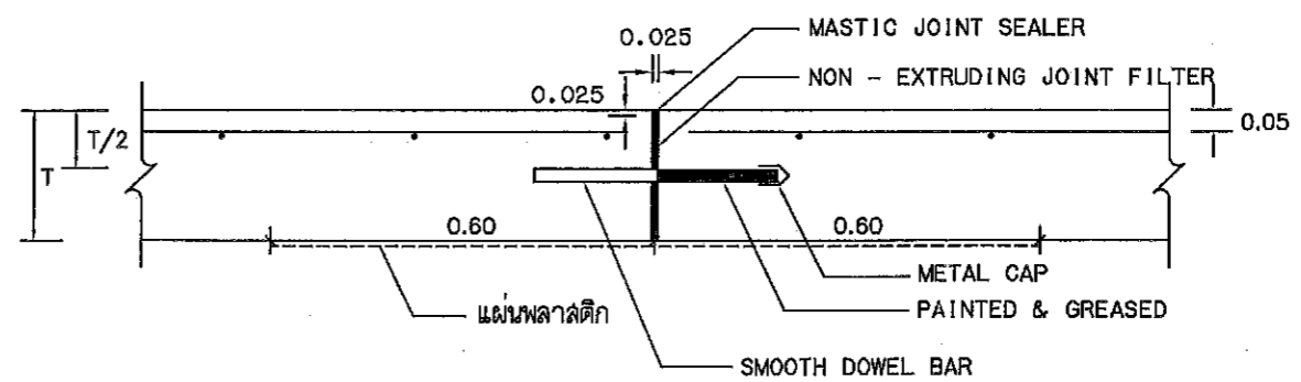
EXPANSION JOINT
